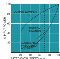
FIGURE 15. ENERGY SAVINGS
