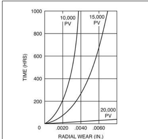
FIGURE 1 — TIME VS. RADIAL WEAR (UNLUBRICATED)
