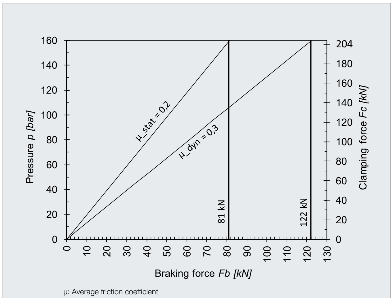
Diagram 1: Pressure-force-diagram
