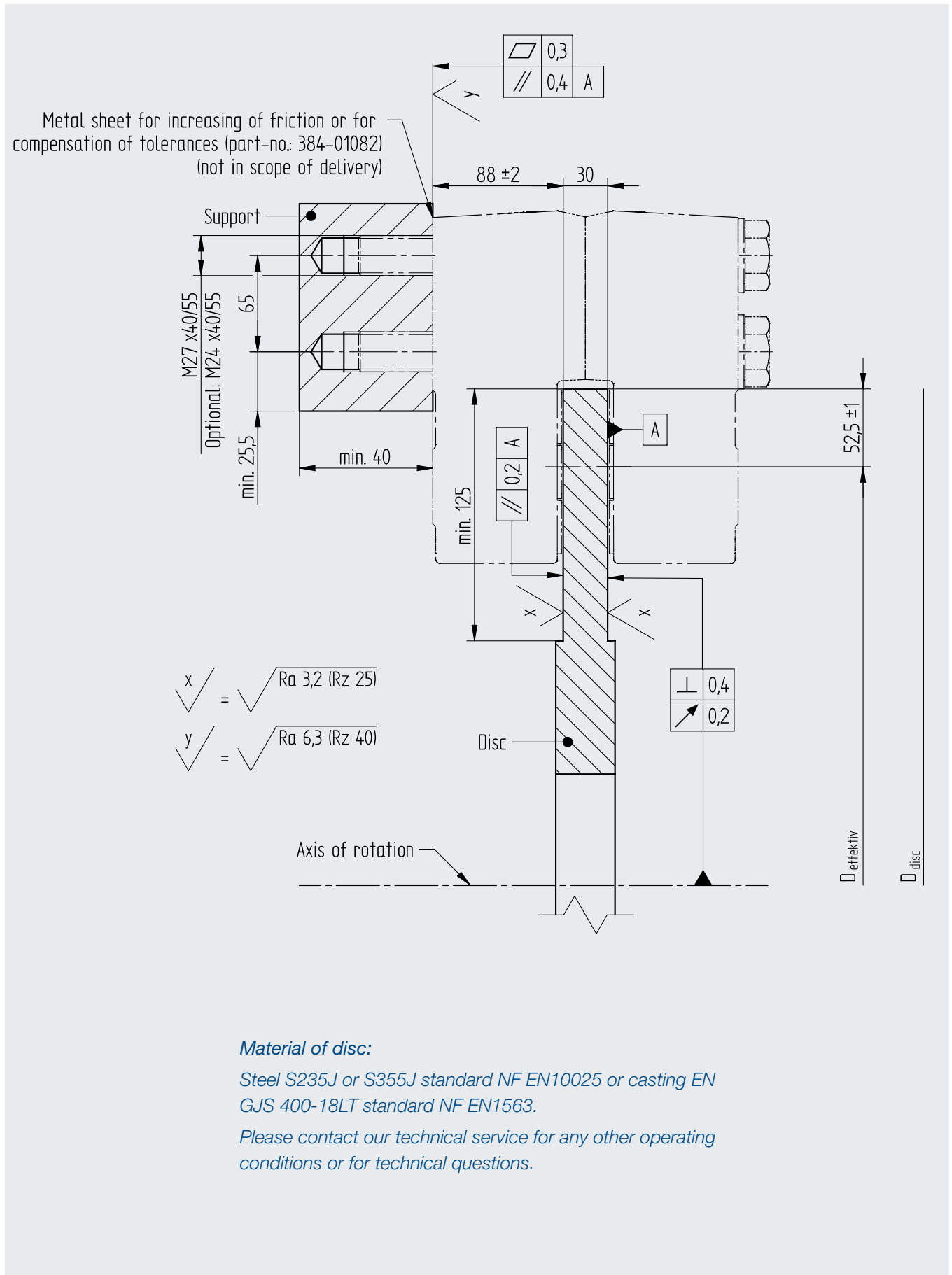
Figure 2: Mounting conditions (sketch is not to scale)
